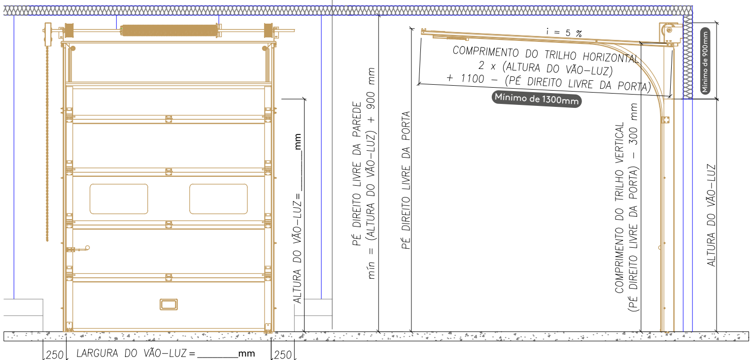
VISTA FRONTAL
