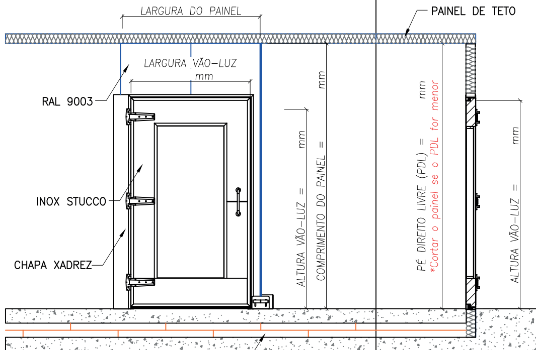
VISTA FRONTAL
