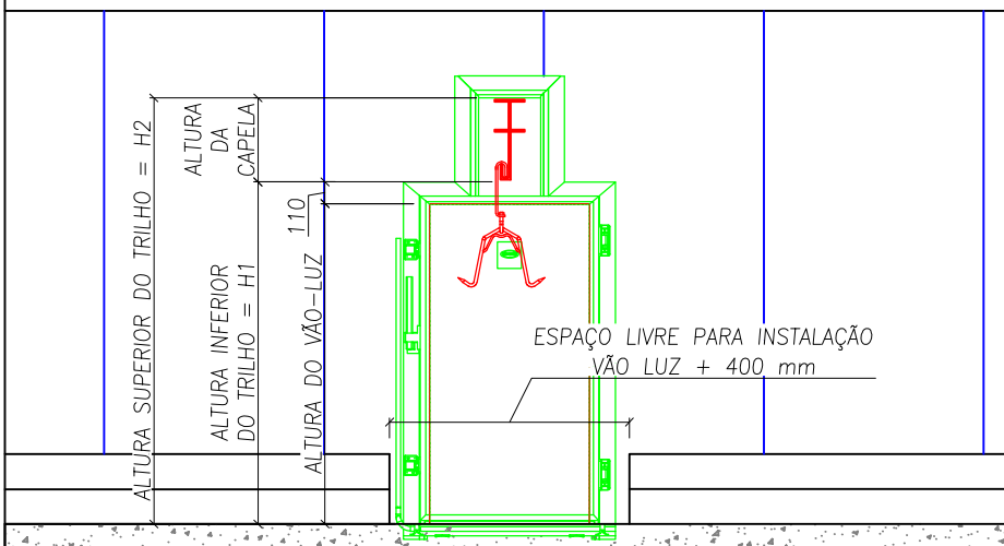
VISTA FRONTAL
