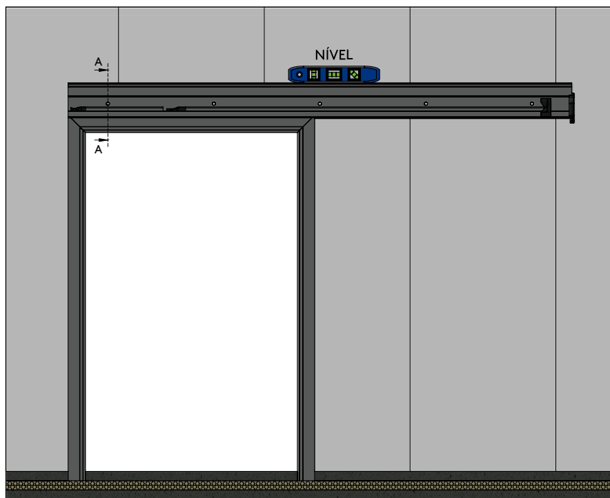
VISTA FRONTAL
