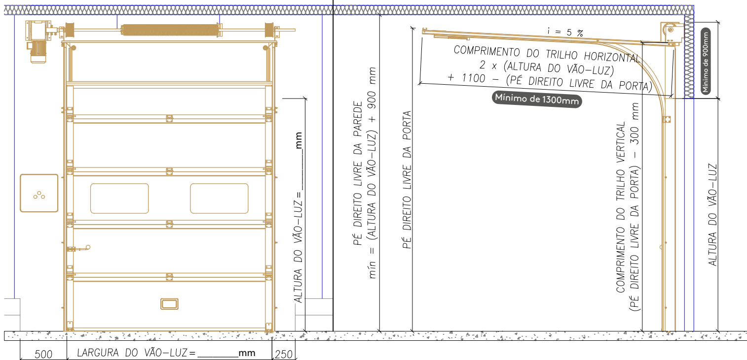
VISTA FRONTAL
